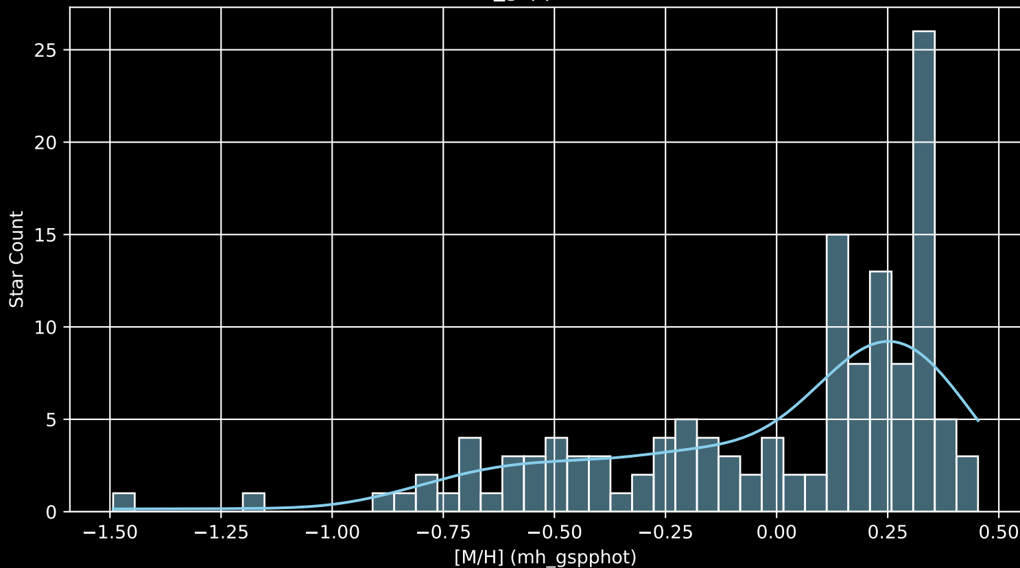
APOGEE DR17 Field: [LMC3 [M/H] (mh_gspphot) (n= 135)
