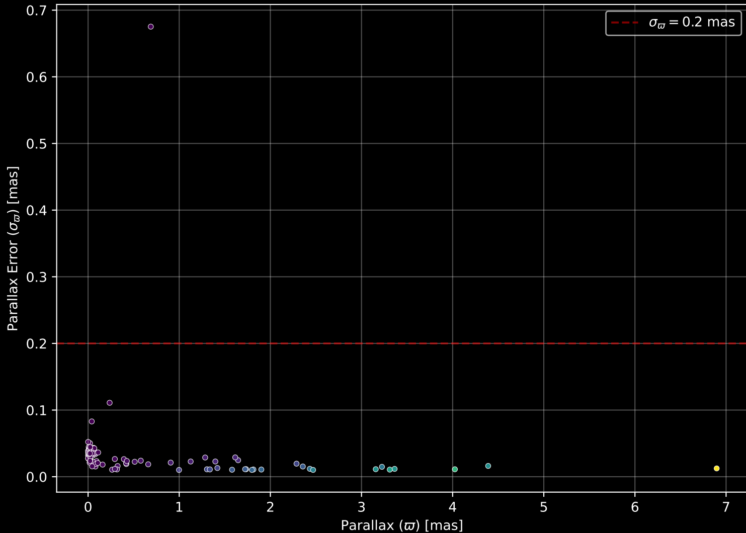
APOGEE DR17 Field: [LMC3] Parallax Quality (n= 140)
