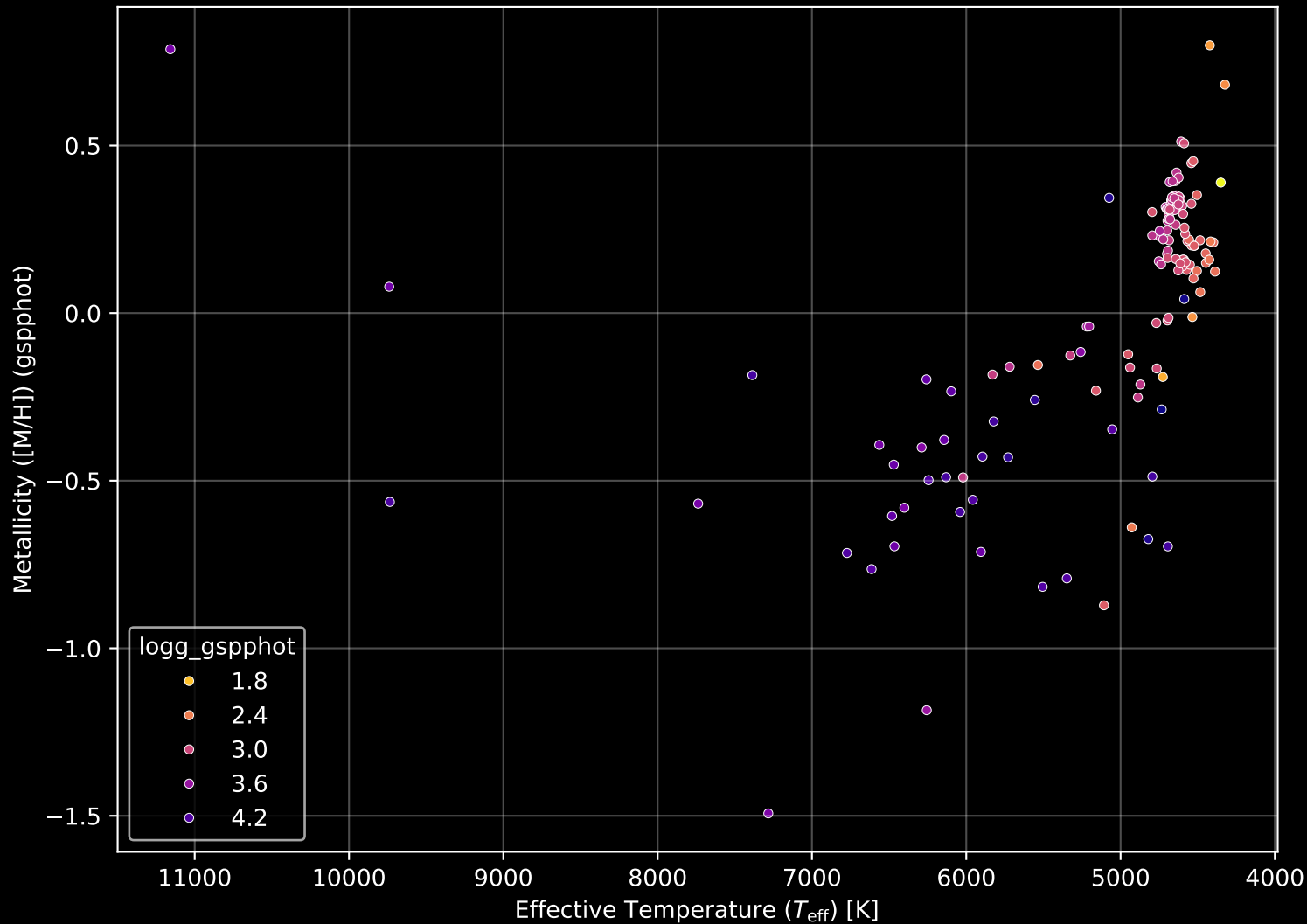
APOGEE DR17 Field: [LMC3] Stellar Population Parameters (n= 140)
