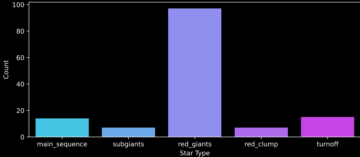
APOGEE DR17 Field: [LMC3] Count plot of Star Type
