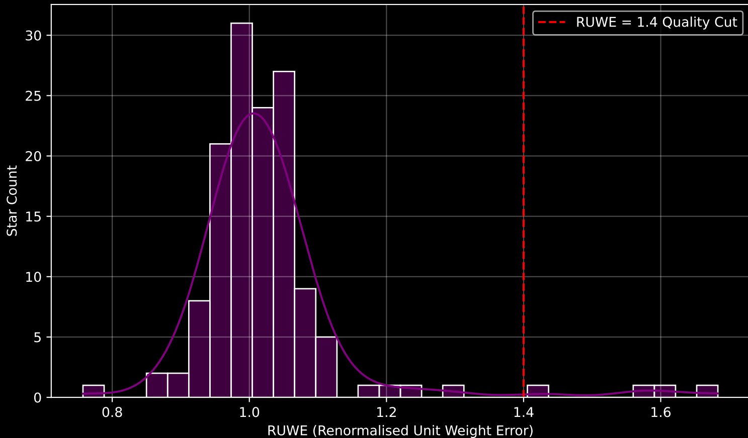
GAPOGEE DR17 Field [LMC3] RUWE Distribution (n= 138)
