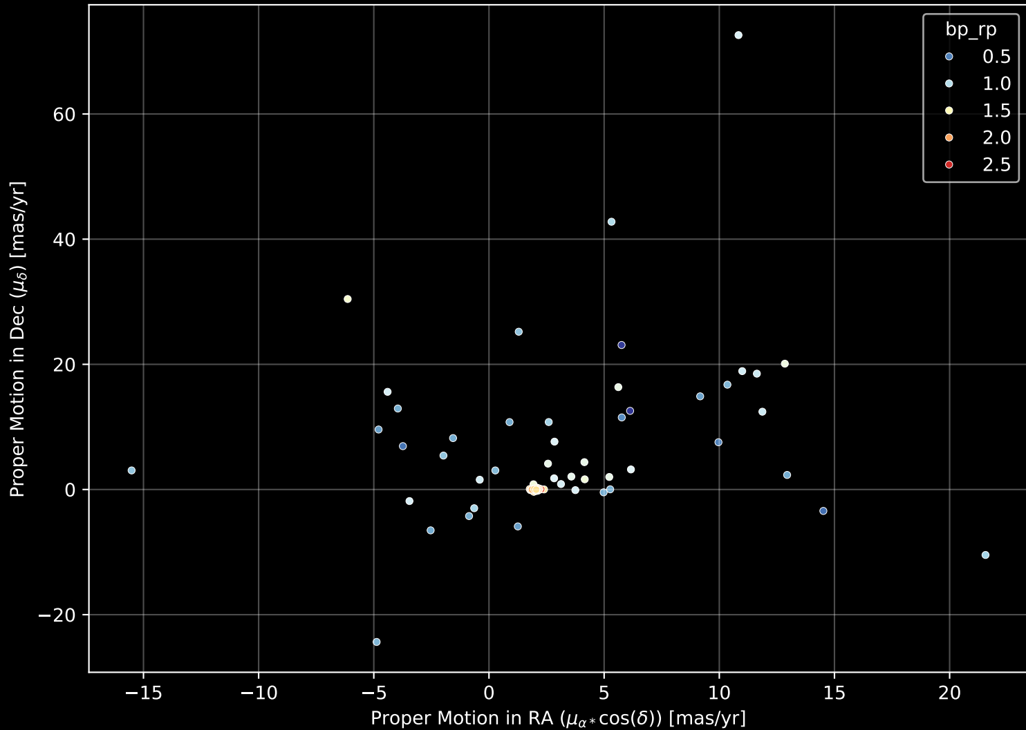
APOGEE DR17 Field: [LMC3] Proper Motion Diagram (n= 140)
