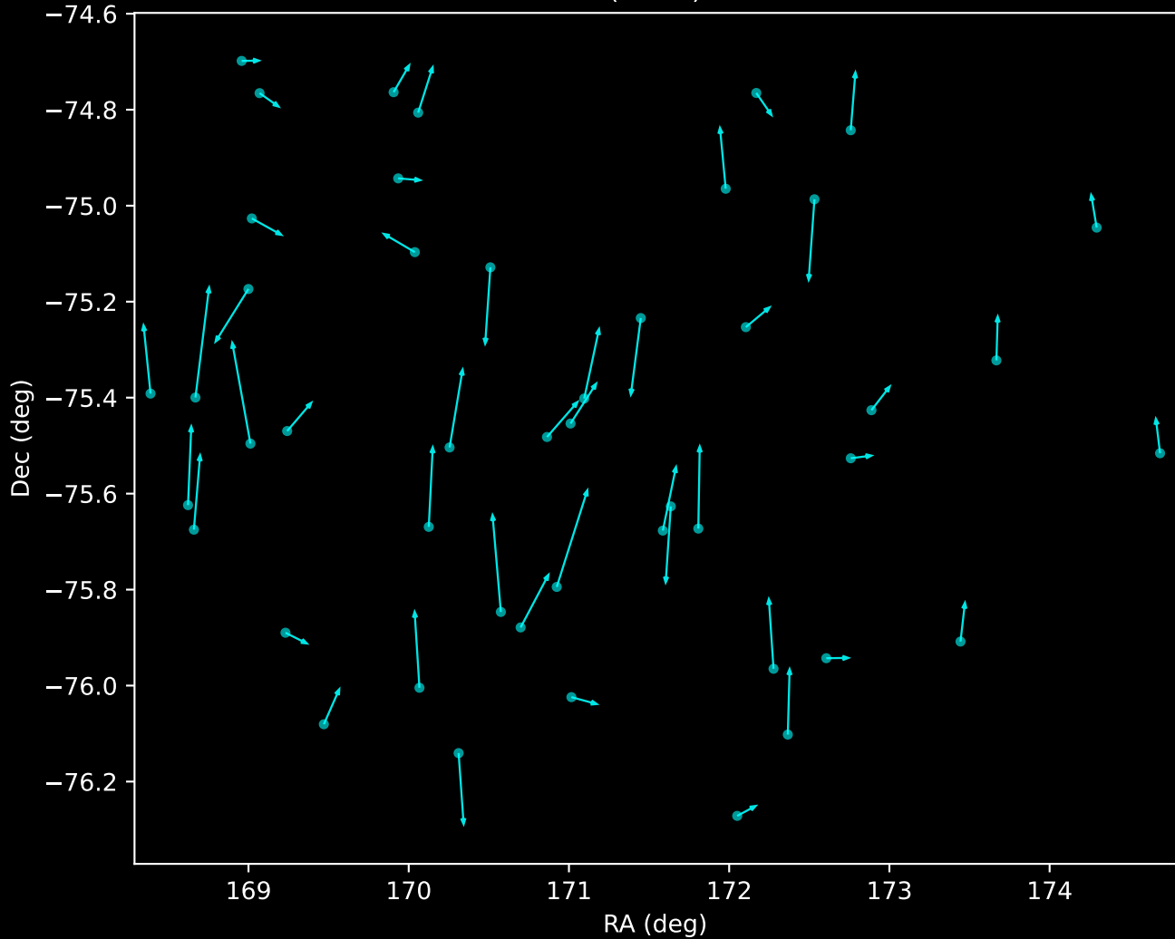
APOGEE DR17 Noise Stream Proper Motion Vectors (n=47)
